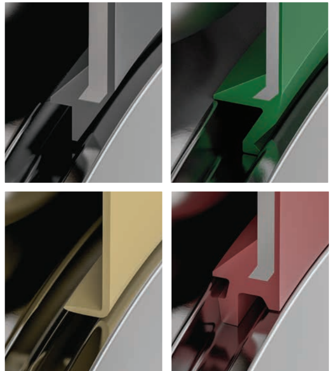
Clockwise from top left: non-contact seal (V), light-contact seal (DW), contact seal (DU), non-contact shield (Z)
